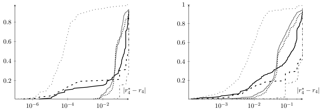
Figure 7. Performance profile with respect to value of the nonlinear parameter r_4 for various starting values for data with (right) and without (left) noise
