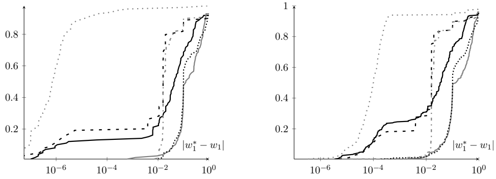
Figure 6. Performance profile with respect to value of the weighting factor w_1 for various starting values for data with (right) and without (left) noise
