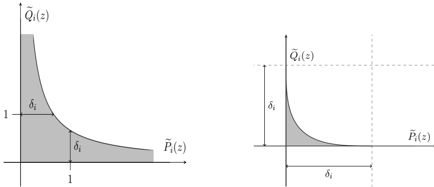
Figure 2. Illustration of the relaxation approach of [56] for one scalar complementarity condition, and of the relaxation approach of [63] for one scalar complementarity condition using the smoothing function \beta_p .
